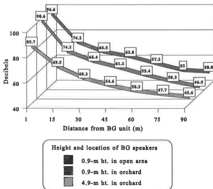
Figure 1. Average sound levels (dB) with increasing distance from a 4-speaker Bird Gard ABC unit at 0.9-m and 4.9-m heights in an almond orchard and in an open area with no obstructions.
