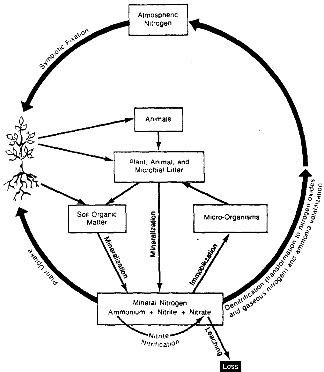
Figure 1. The nitrogen cycle. (Adapted from Reeder and Sabey 1987)
