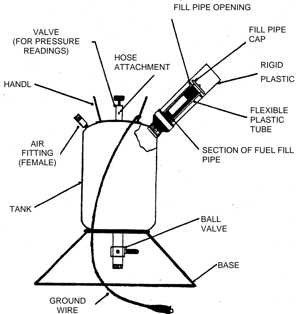
FIGURE 1: Field Compliance Test Unit
