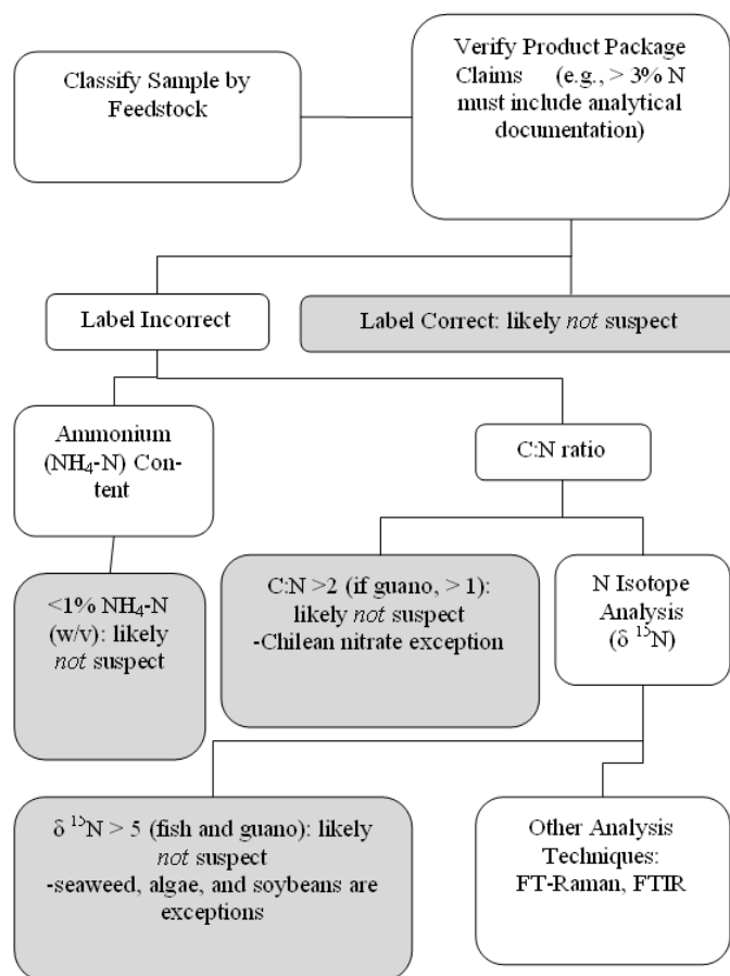
Figure 10. Flow chart showing the tests in the protocol to determine the potential adulteration of organic fertilizers
