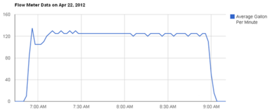
Figure 3. Display of flow meter data for a single irrigation event.
