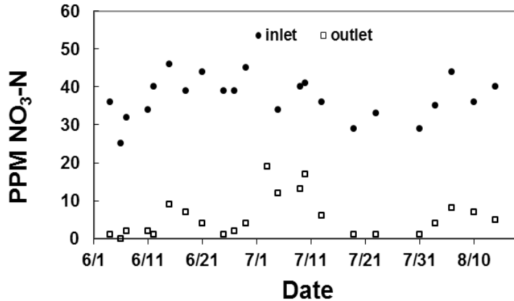
Figure 3. Reduction of water \text{NO}_3\text{-N} concentration in the denitrification bioreactor treating surface runoff (site 3).
