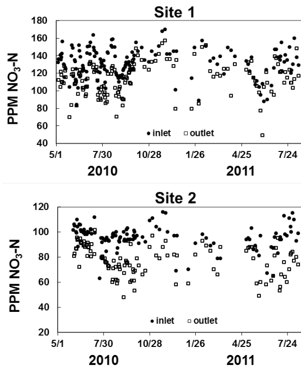
Figure 2. Reduction of water \text{NO}_3\text{-N} concentration in denitrification bioreactors treating tile drain effluent.
