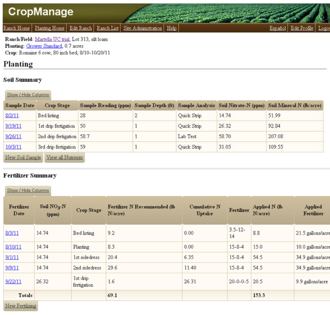
Figure 1. Example display of the soil test and the fertilizer summaries for a romaine lettuce crop.
