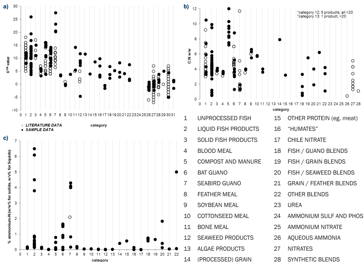
Figure 1. Graphical summary for a) the nitrogen isotope ratios; b) C:N and c) % ammonium -N content data compiled from literature and analysis of organic fertilizer samples.
