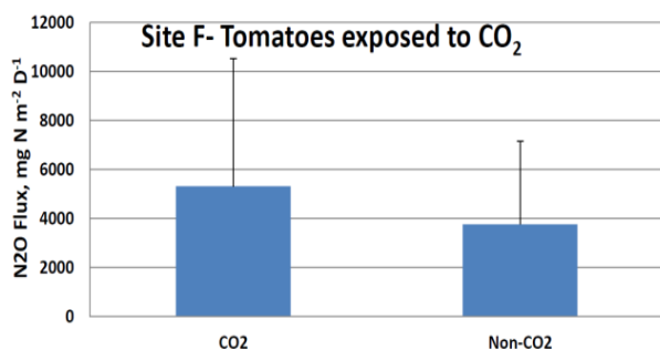
Figure 5. Example of N 2 O fluxes measured in tomatoes exposed to elevated CO 2 levels.
