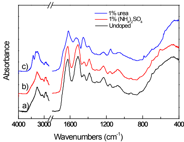
Figure 2. ATR-FTIR spectra of bloodmeal fertilizer a) undoped; b) doped with 1% ammonium sulfate and c) doped with 1% urea.
