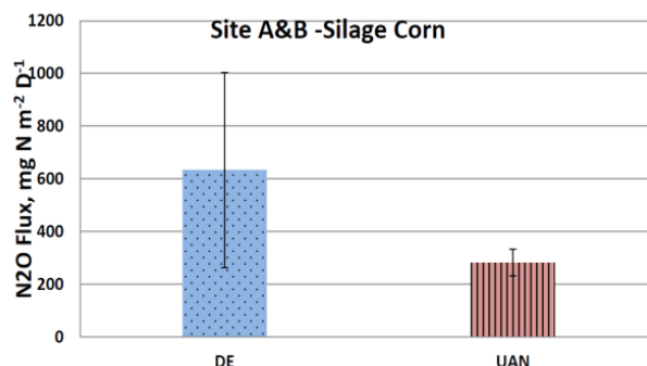
Figure 1. Example of N 2 O fluxes measured at site A & B -Silage corn in Hanford.
