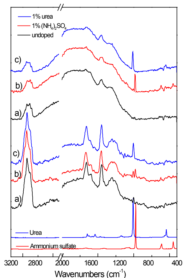
Figure 6. FT-Raman spectra of two feathermeal fertilizers a) undoped; b) doped with 1% ammonium sulfate and c) doped with 1% urea.
