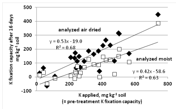
Figure 1. Change in soil K fixation capacity following KCl application. Samples are described in Table 1. Samples were incubated moist for 16 days following K application, then analyzed without drying (squares) or after air drying (diamonds). Applying K to samples in amounts equal to initial Kfix reduced K fixation, but not to zero.
