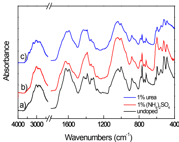
Figure 4. ATR-FTIR spectra of seabird guano fertilizer a) undoped; b) doped with 1% ammonium sulfate and c) doped with 1% urea.
