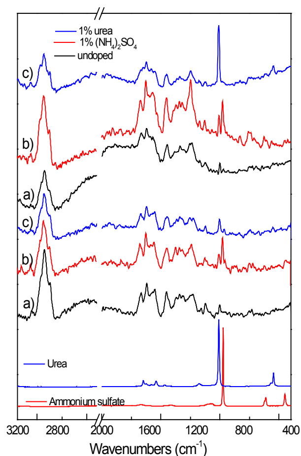
Figure 7. FT-Raman spectra of two bloodmeal fertilizers a) undoped; b) doped with 1% ammonium sulfate and c) doped with 1% urea.
