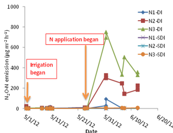
Figure 7. N 2 O emission rates from May 1 through June 12, 2012.
