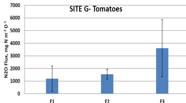
Figure 6. Example of N 2 O fluxes measured for tomatoes fertilized with 100 (F1), 150(F2) and 200 (F3) lbs of N/ac during the season and irrigated with subsurface drip irrigation.
