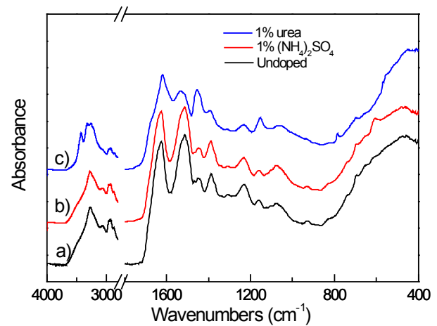
Figure 5. ATR-FTIR spectra of compost fertilizer a) undoped; b) doped with 1% ammonium sulfate and c) doped with 1% urea.
