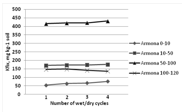
Figure 2. Kfix values for the Armona loam soil after 1, 2, 3, and 4 cycles of wetting and drying. Soil Kfix did not change significantly with additional wet/dry cycles.
