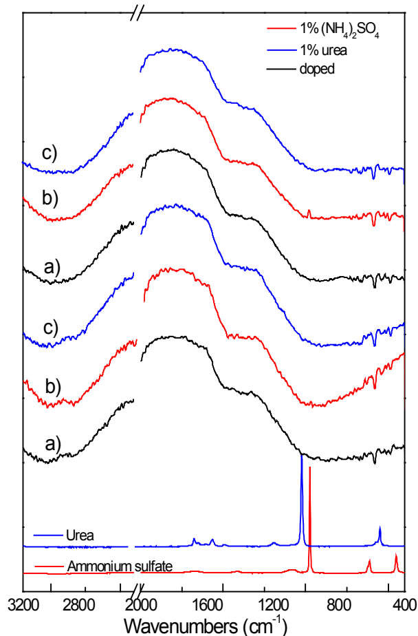
Figure 9. FT Raman spectra of two compost fertilizers a) undoped; b) doped with 1% ammonium sulfate and c) doped with 1% urea.
