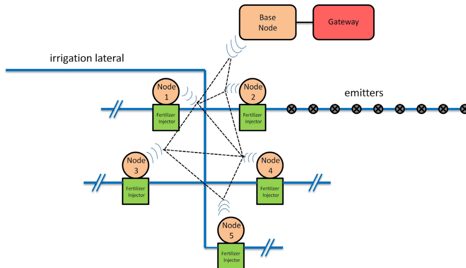
Figure 4. Wireless network for controlled fertigation.
