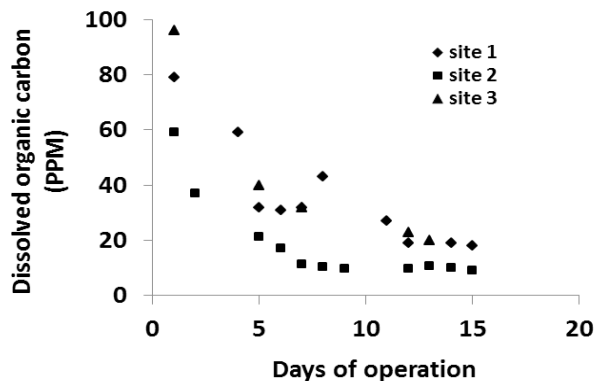
Figure 1. Dissolved organic carbon concentration of denitrification bioreactor effluent in the initial weeks of operation.
