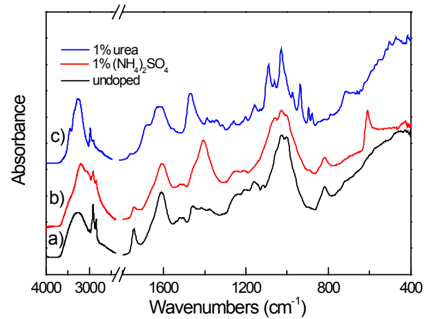
Figure 3. ATR-FTIR spectra of seaweed fertilizer a) undoped; b) doped with 1% ammonium sulfate and c) doped with 1% urea.
