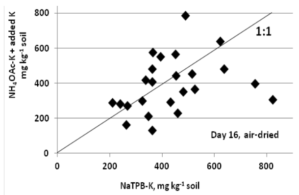
Figure 3. NaTPB-extractable K vs. previously measured (initial) NH 4 OAc-extractable K + K added in treatment (Day 16, air-dried). Most TPB-K levels after drying were lower than [Initial TPB-K + added K], indicating that some of the added K was not only fixed but also removed from the pool of plant-available K.
