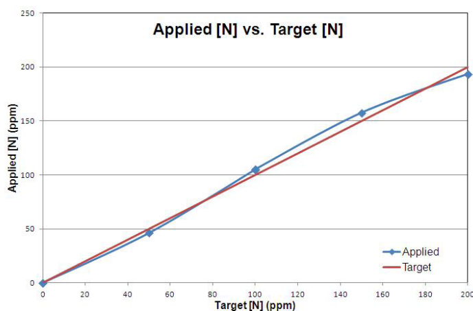
Figure 3. Target and measured nitrogen concentrations of fertilizer solutions delivered by adjustment of duty cycle to venturi suction valve.
