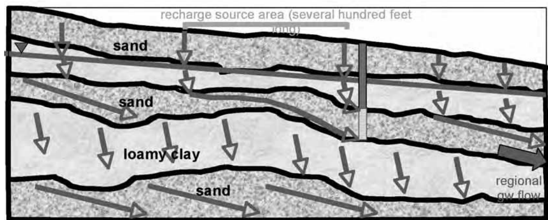
Figure 1 Monitoring in Heterogeneous Aquifer
