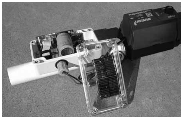
Figure 2 a, b First and second generation wireless valve controllers.
