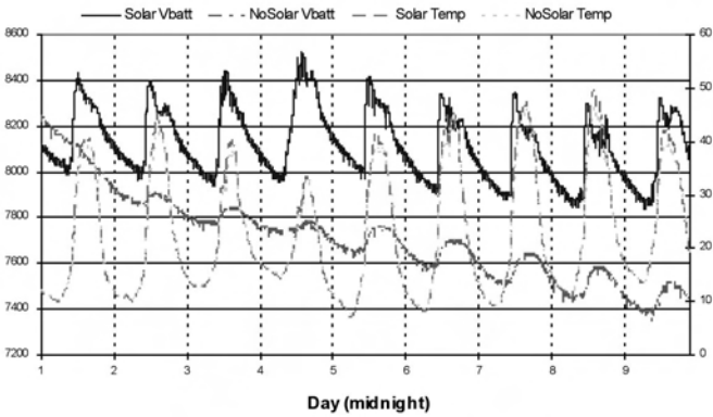
Figure 4 Battery voltage and temperature inside valve controller enclosures over 9 days.
