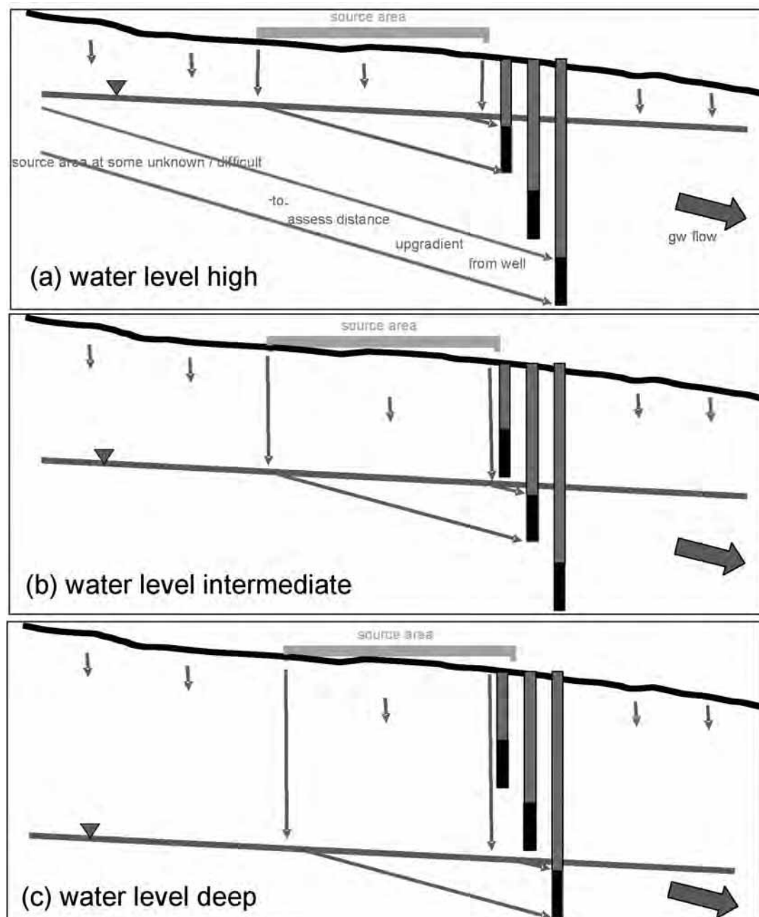
Figure 2 Monitoring a Dynamic Water Table
