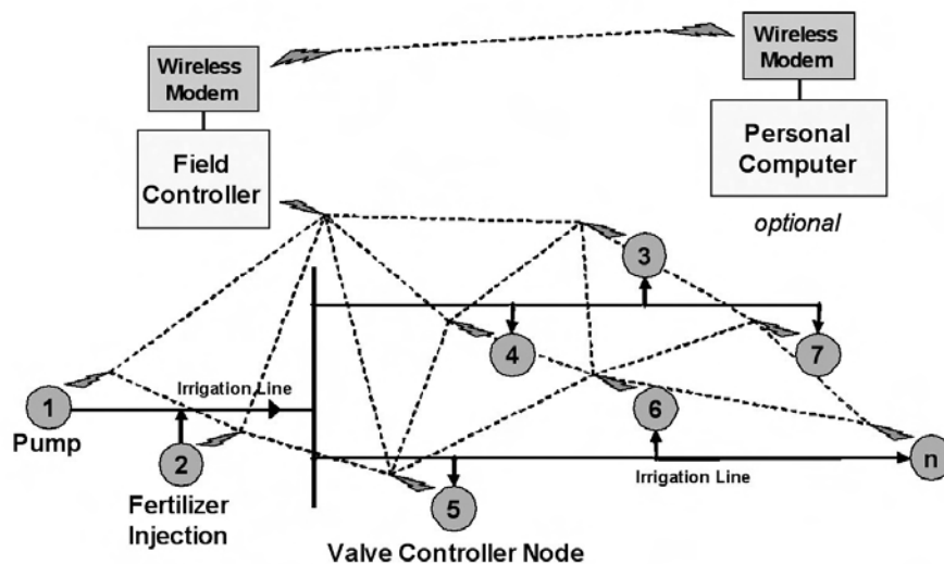
Figure 1 Layout of wireless valve network.
