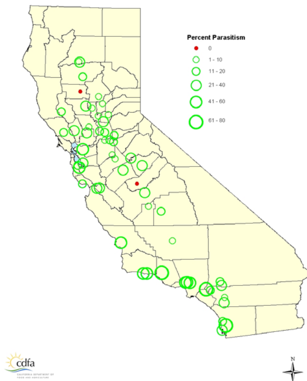
Figure 2. Percent of lerps with parasitoid exit holes. Fall 2003 survey by the CDFA Biological Control Program .
